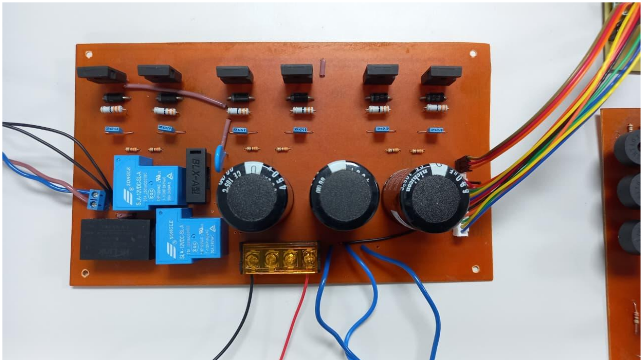
Figure 10: Hardware circuit - Inverter circuit
