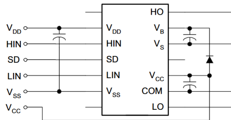
Figure 5: Gate driver circuit
