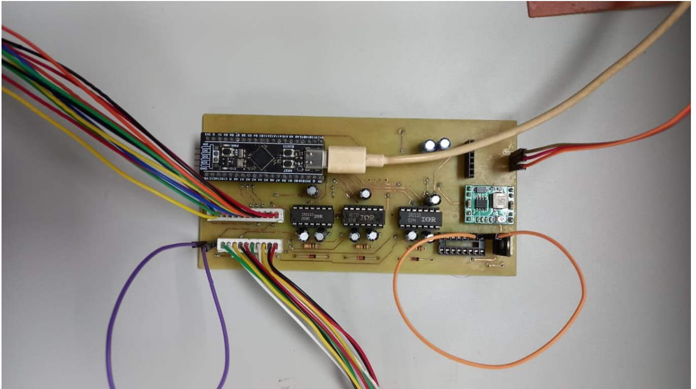
Figure 4: Hardware - Controller circuit
