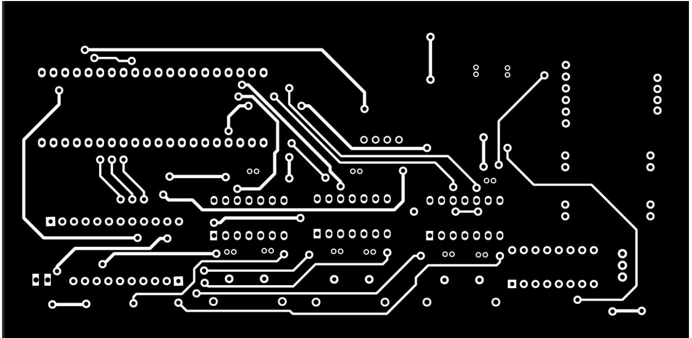
Figure 2: Controller circuit : PCB : Layer 1
