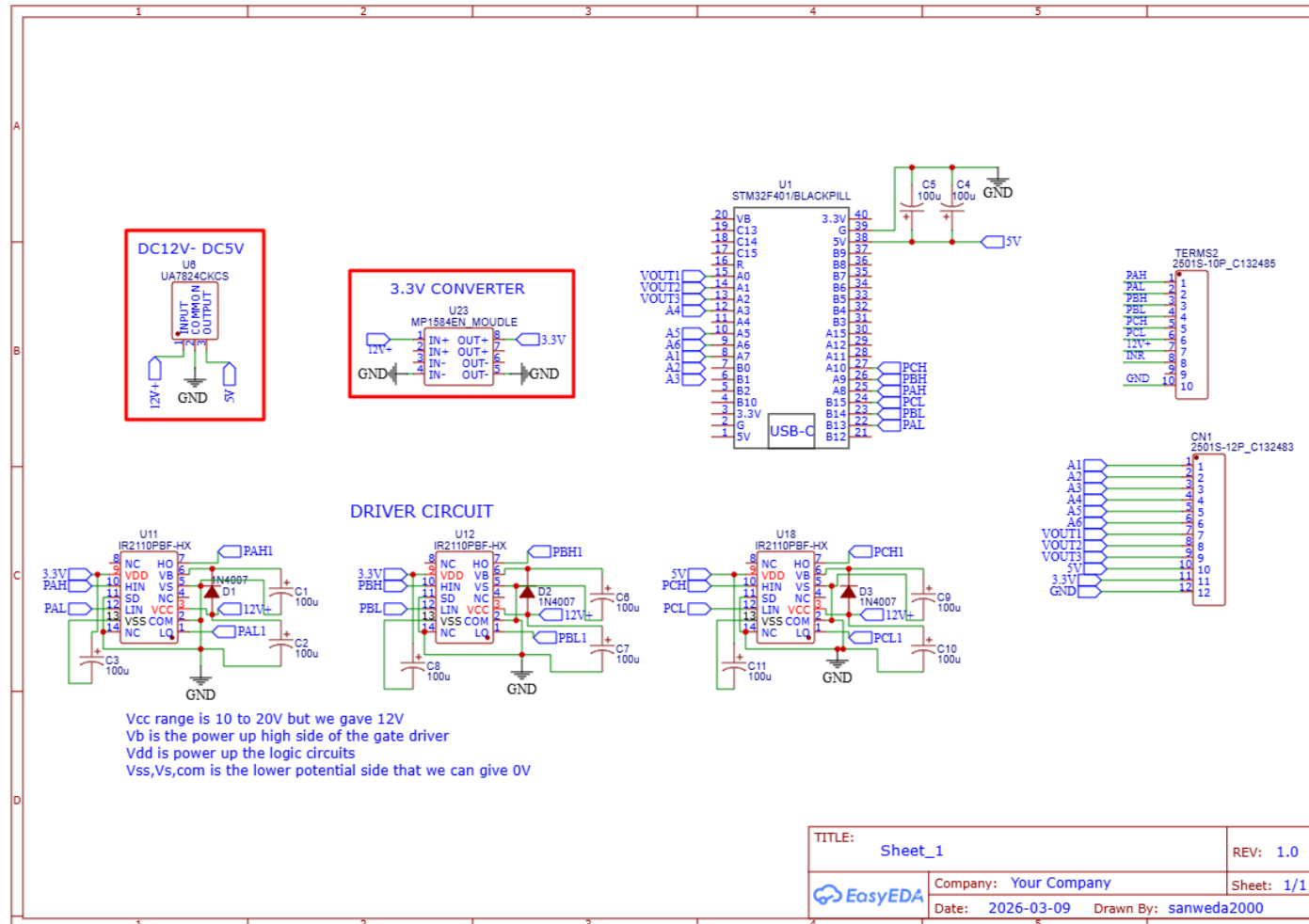
Figure 1: Schematic diagram of Controlling circuit
