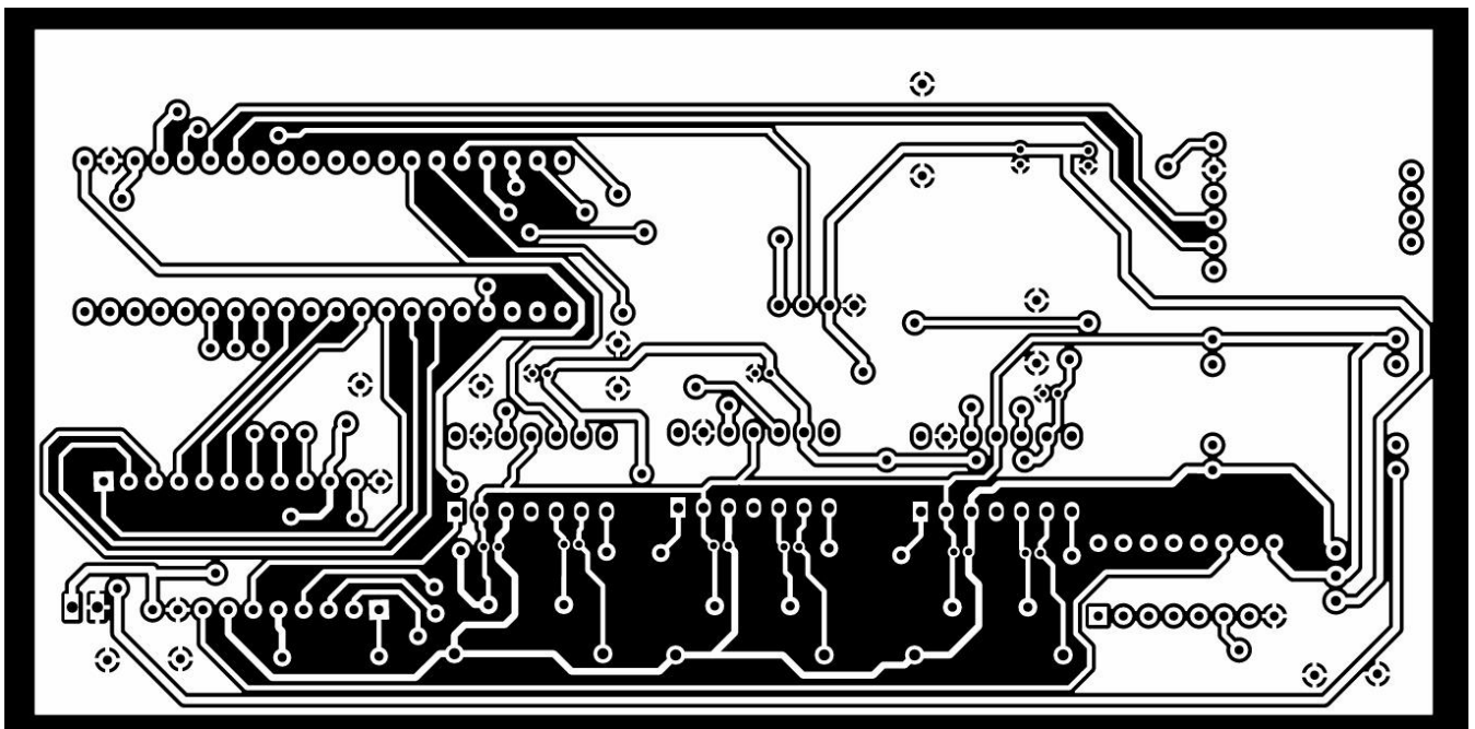
Figure 3: Controller circuit : PCB : Layer 2
