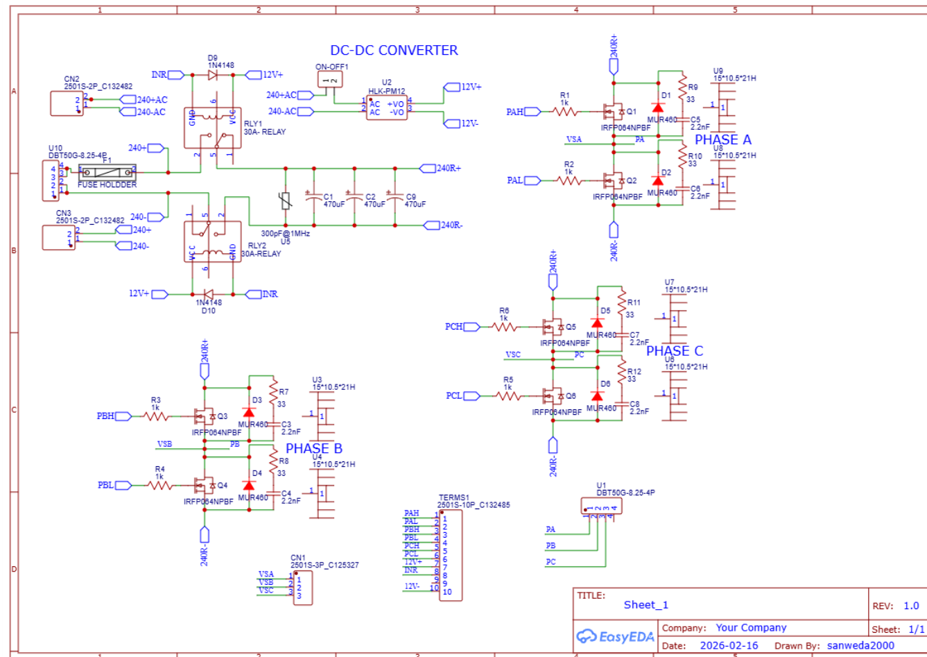
Figure 8: Schematic diagram of Inverter circuit
