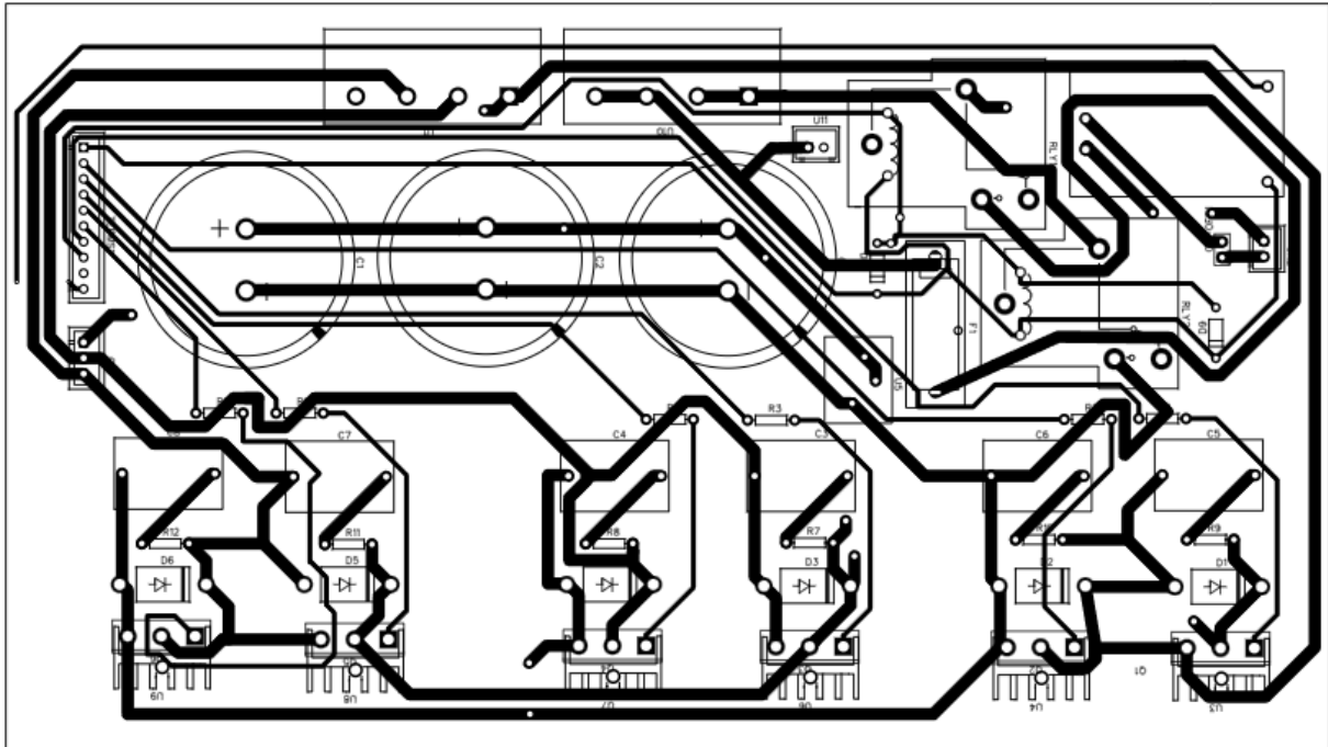
Figure 9: PCB design of Inverter circuit
