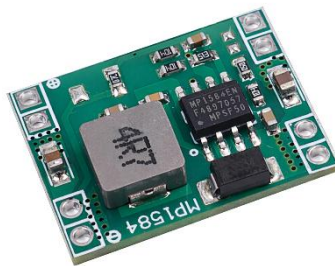
Figure 6: MP1584EN DC-DC buck converter
